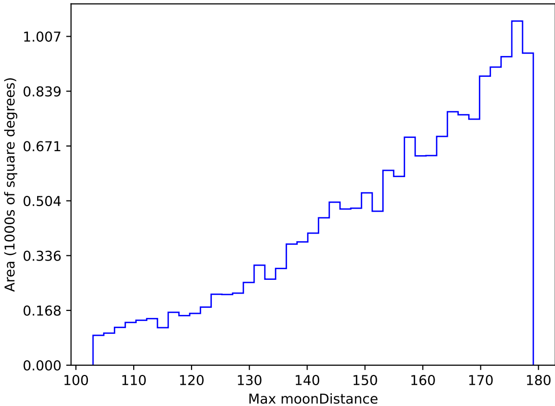
ddf_loaded_half_fl15_v3.4_10yrs WFD g band: Max moonDistance
