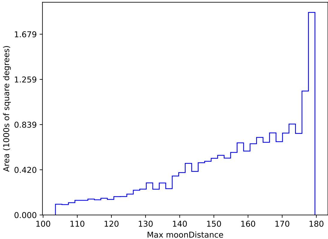
ddf_loaded_half_fl15_v3.4_10yrs WFD all bands: Max moonDistance
