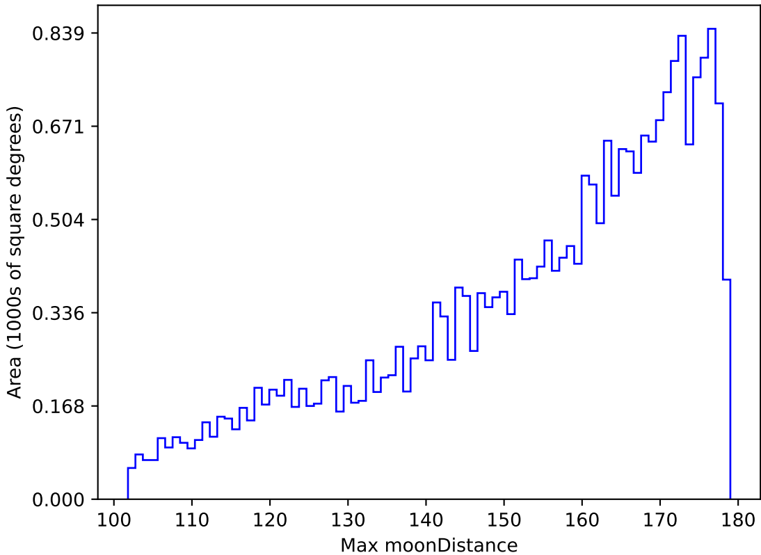
ddf_loaded_half_fl15_v3.4_10yrs All sky z band: Max moonDistance
