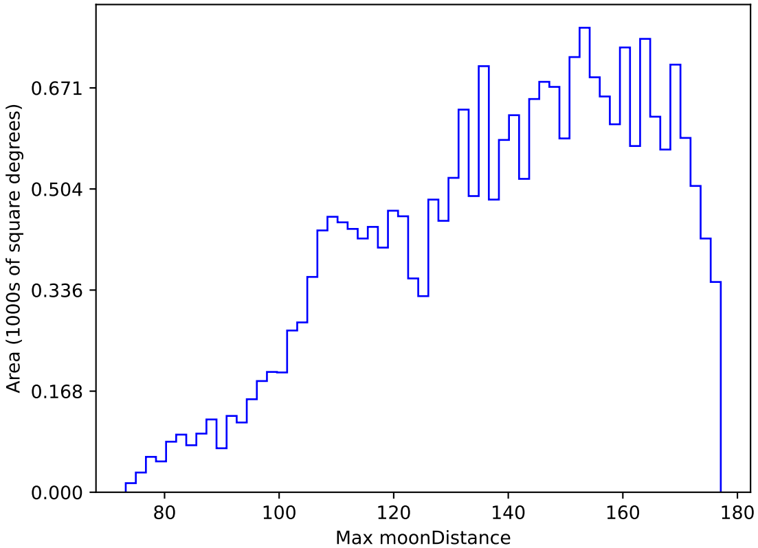
ddf_loaded_half_fl15_v3.4_10yrs All sky y band: Max moonDistance
