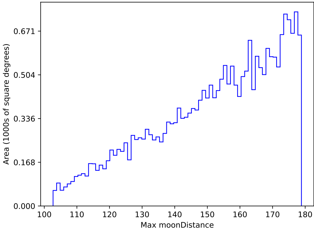
ddf_loaded_half_fl15_v3.4_10yrs All sky u band: Max moonDistance
