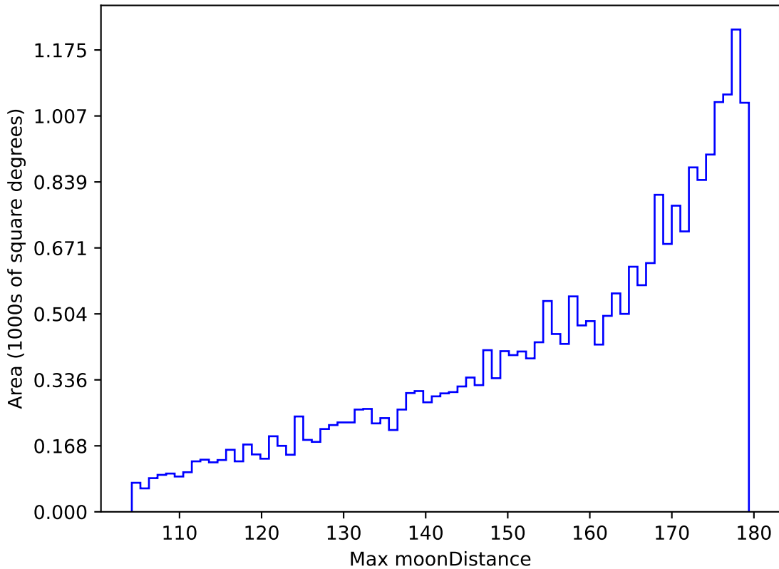
ddf_loaded_half_fl15_v3.4_10yrs All sky r band: Max moonDistance
