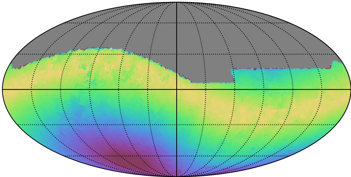
ddf_loaded_half_fl15_v3.4_10yrs All sky i band: Max moonDistance
