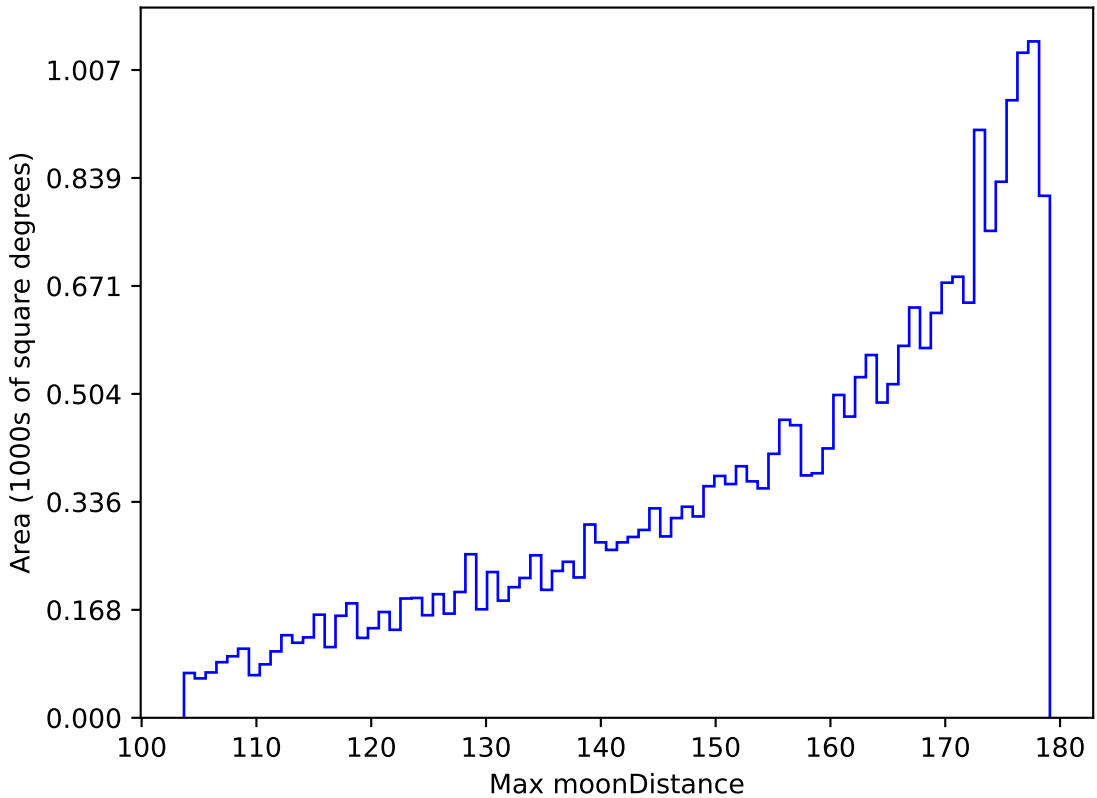
ddf_loaded_half_fl15_v3.4_10yrs All sky i band: Max moonDistance
