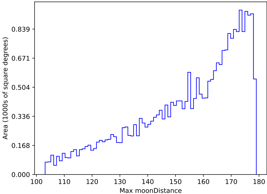
ddf_loaded_half_fl15_v3.4_10yrs All sky g band: Max moonDistance
