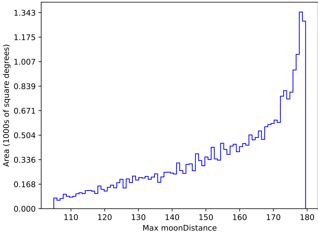
ddf_loaded_half_fl15_v3.4_10yrs All sky all bands: Max moonDistance
