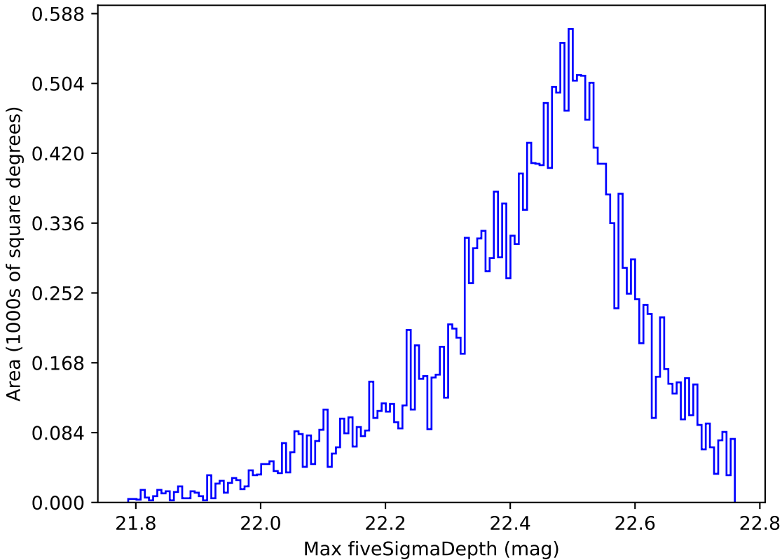
ddf_loaded_half_fl15_v3.4_10yrs Yr 1 y band: Max fiveSigmaDepth
