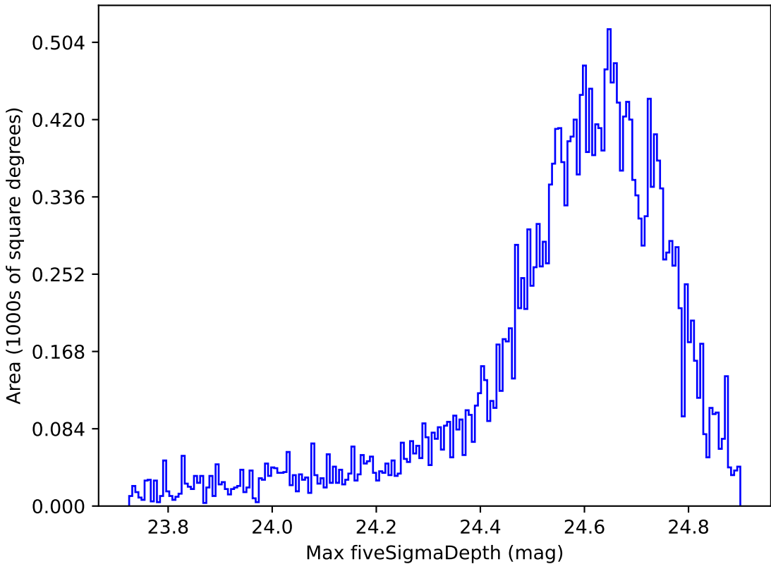
ddf_loaded_half_fl15_v3.4_10yrs Yr 1 r band: Max fiveSigmaDepth
