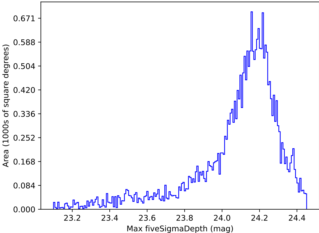
ddf_loaded_half_fl15_v3.4_10yrs Yr 1 i band: Max fiveSigmaDepth
