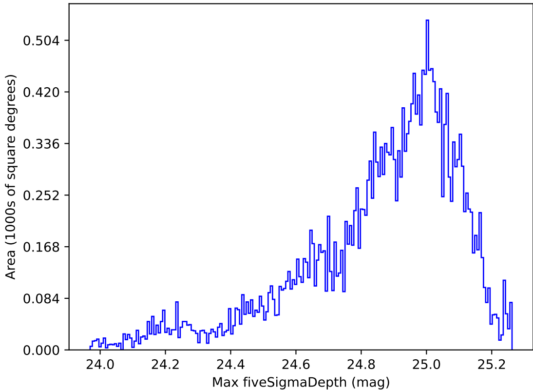
ddf_loaded_half_fl15_v3.4_10yrs Yr 1 g band: Max fiveSigmaDepth
