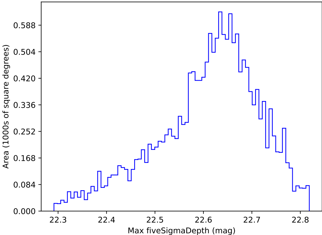
ddf_loaded_half_fl15_v3.4_10yrs WFD y band: Max fiveSigmaDepth
