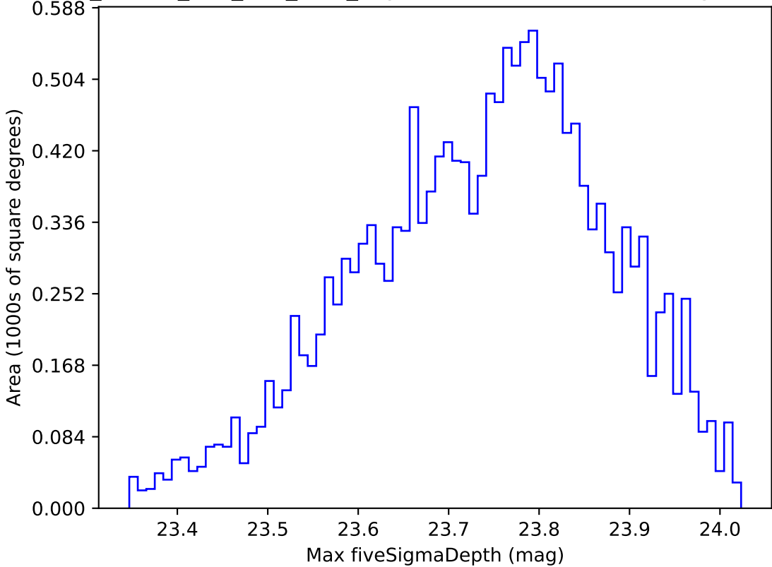
ddf_loaded_half_fl15_v3.4_10yrs WFD u band: Max fiveSigmaDepth
