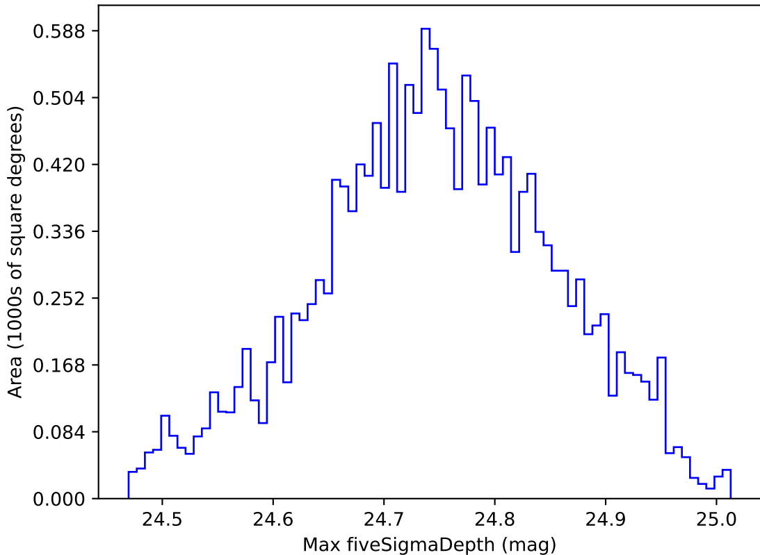
ddf_loaded_half_fl15_v3.4_10yrs WFD r band: Max fiveSigmaDepth
