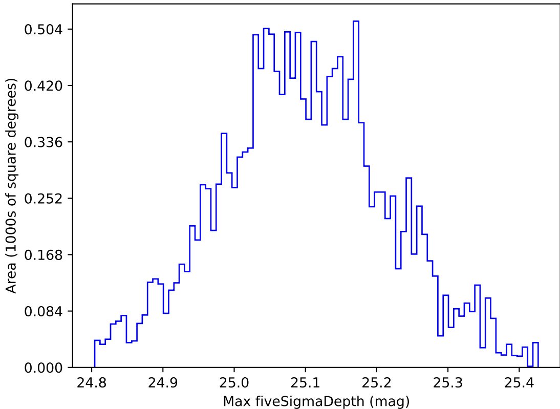
ddf_loaded_half_fl15_v3.4_10yrs WFD all bands: Max fiveSigmaDepth
