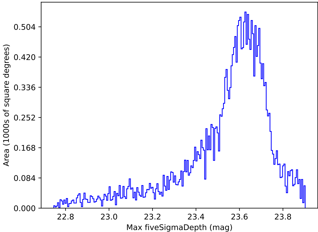
ddf_loaded_half_fl15_v3.4_10yrs All sky z band: Max fiveSigmaDepth
