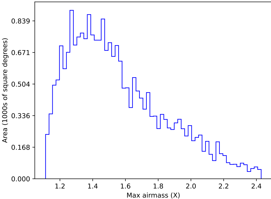
ddf_loaded_half_f15_v3.4_10yrs Yr 1 u band: Max airmass
