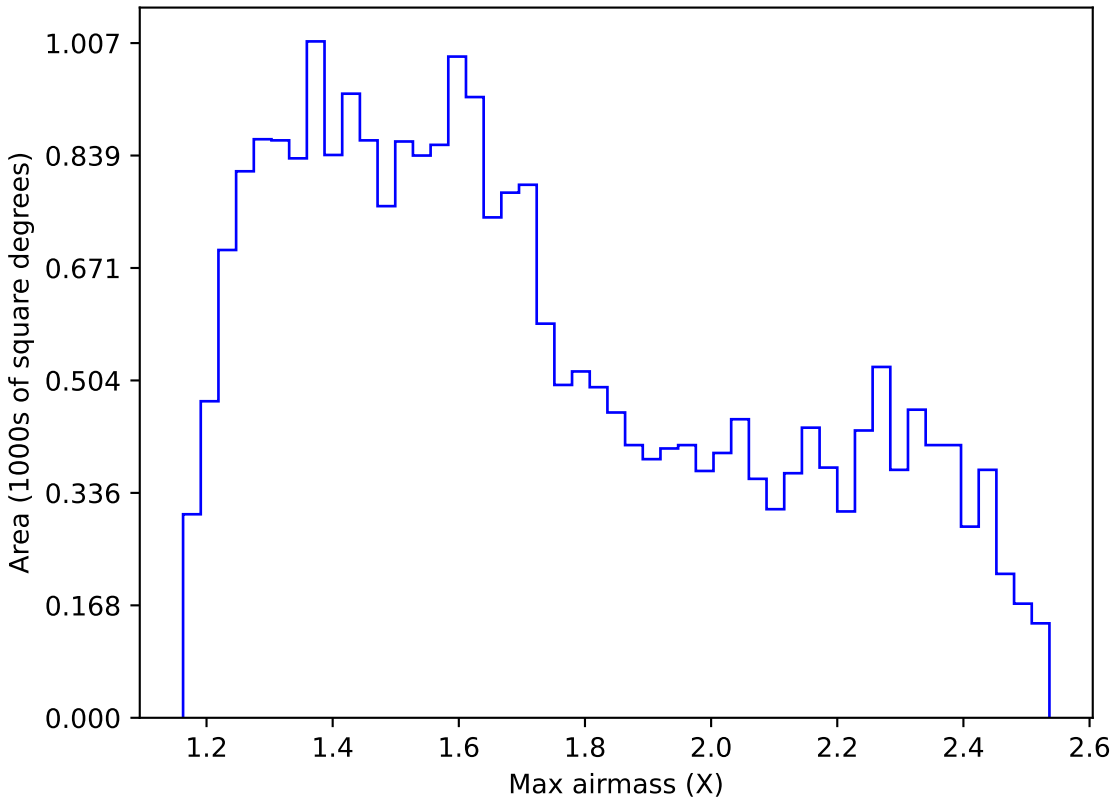
ddf_loaded_half_fl15_v3.4_10yrs Yr 1 r band: Max airmass
