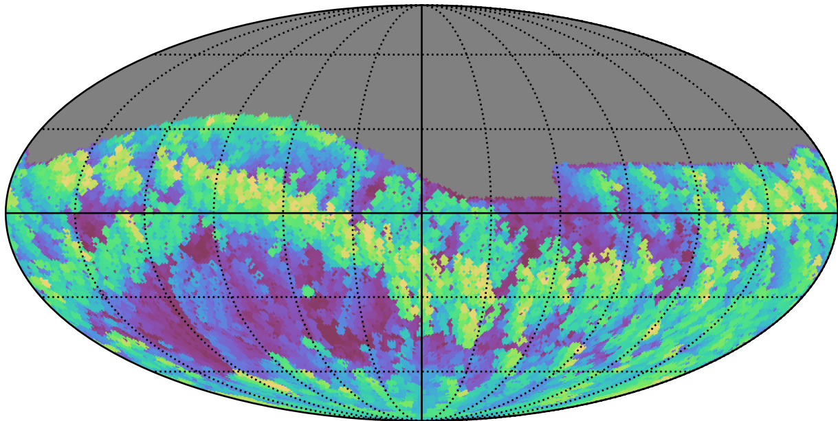
ddf_loaded_half_fl15_v3.4_10yrs Yr 1 all bands: Max airmass
