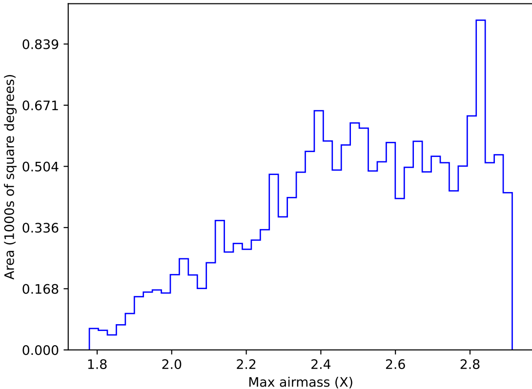
ddf_loaded_half_fl15_v3.4_10yrs WFD z band: Max airmass
