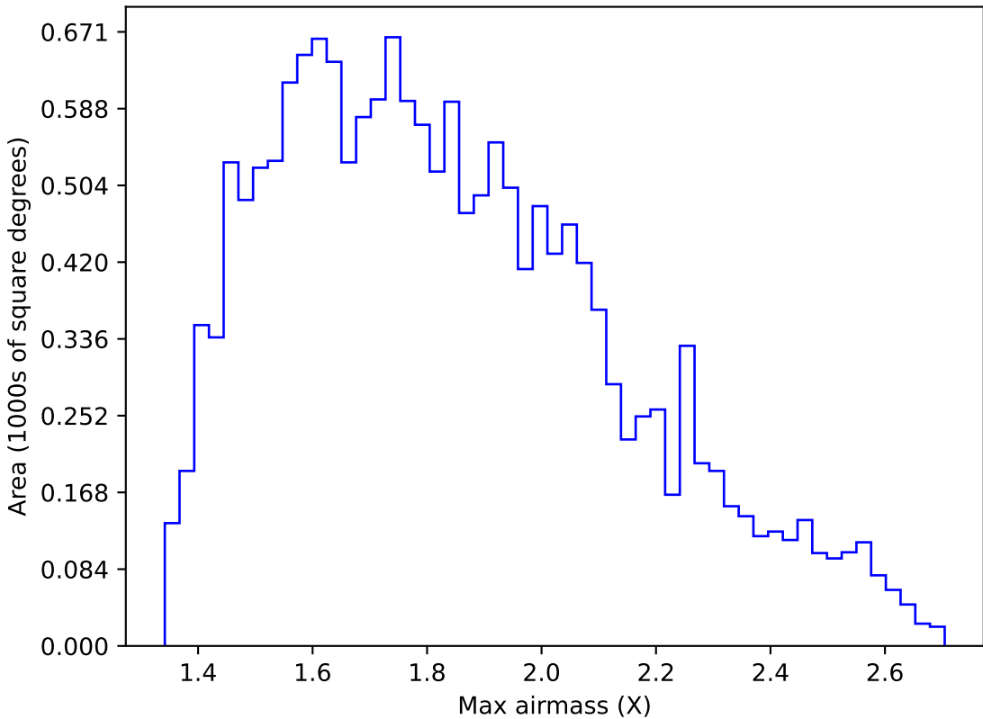
ddf_loaded_half_fl15_v3.4_10yrs WFD u band: Max airmass
