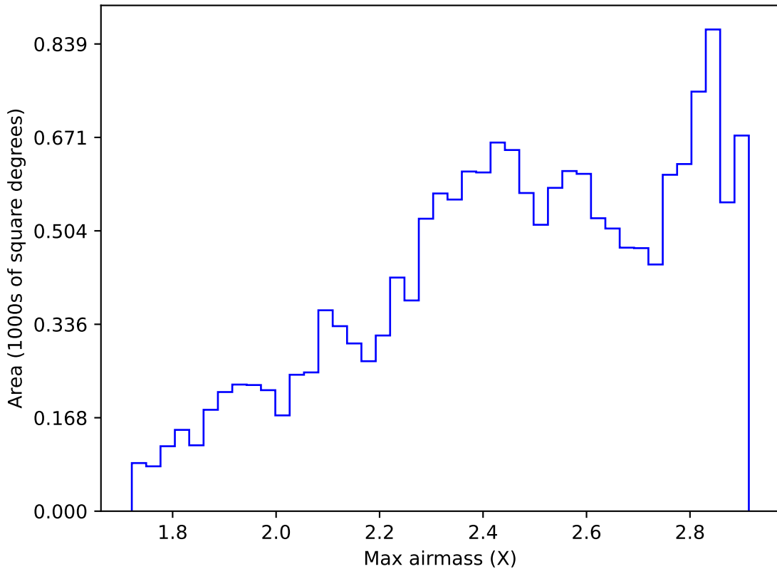
ddf_loaded_half_f15_v3.4_10yrs WFD i band: Max airmass
