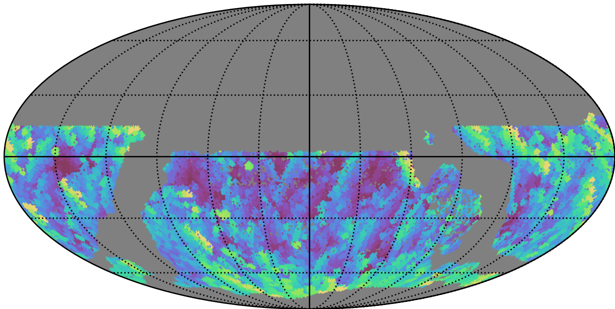
ddf_loaded_half_fl15_v3.4_10yrs WFD g band: Max airmass
