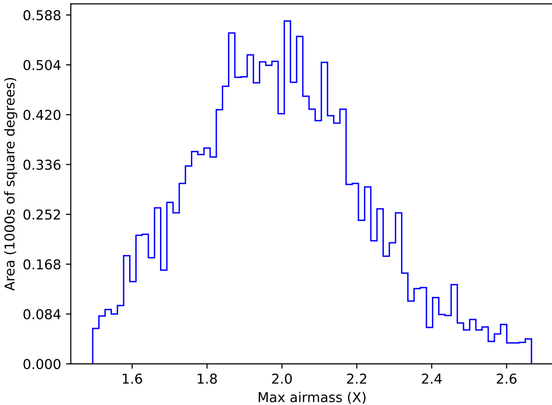
ddf_loaded_half_fl15_v3.4_10yrs WFD g band: Max airmass
