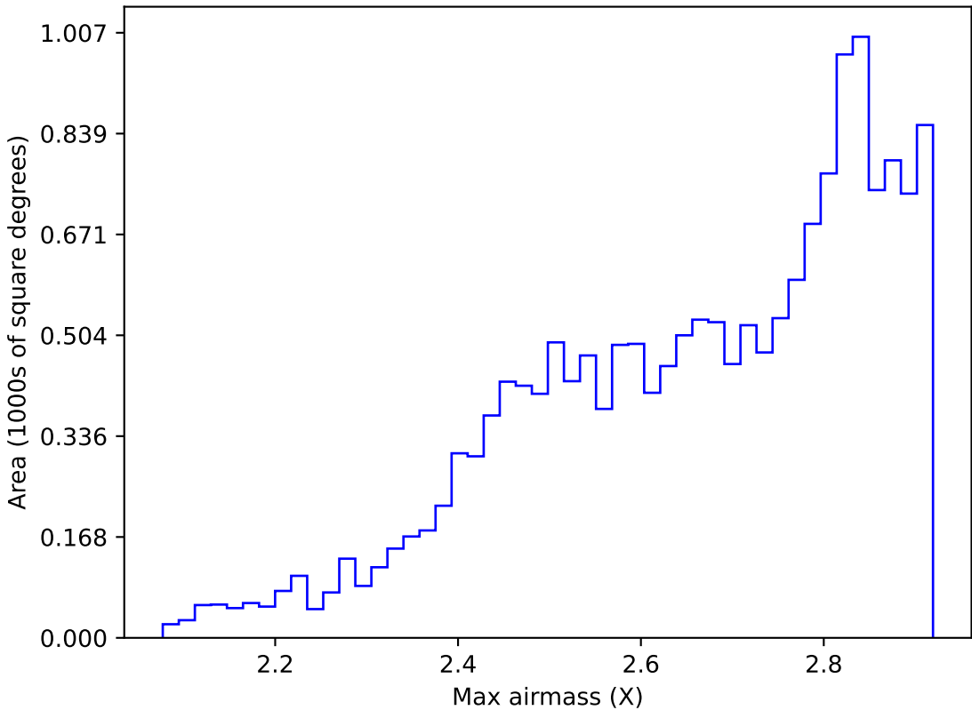
ddf_loaded_half_fl15_v3.4_10yrs WFD all bands: Max airmass
