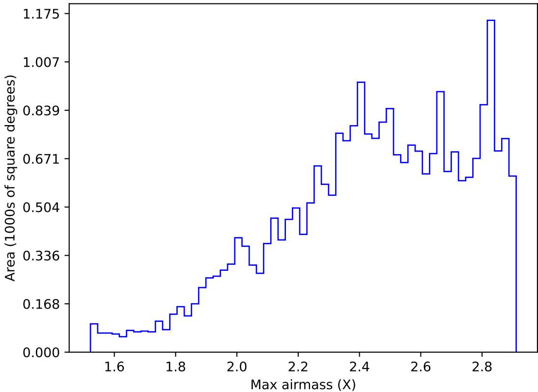
ddf_loaded_half_fl15_v3.4_10yrs All sky z band: Max airmass
