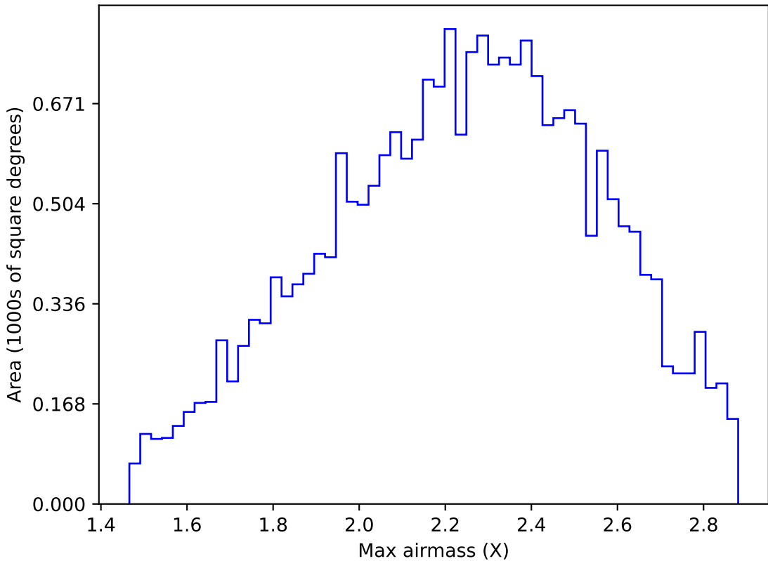
ddf_loaded_half_fl15_v3.4_10yrs All sky y band: Max airmass
