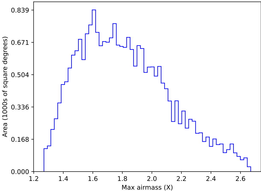
ddf_loaded_half_fl15_v3.4_10yrs All sky u band: Max airmass
