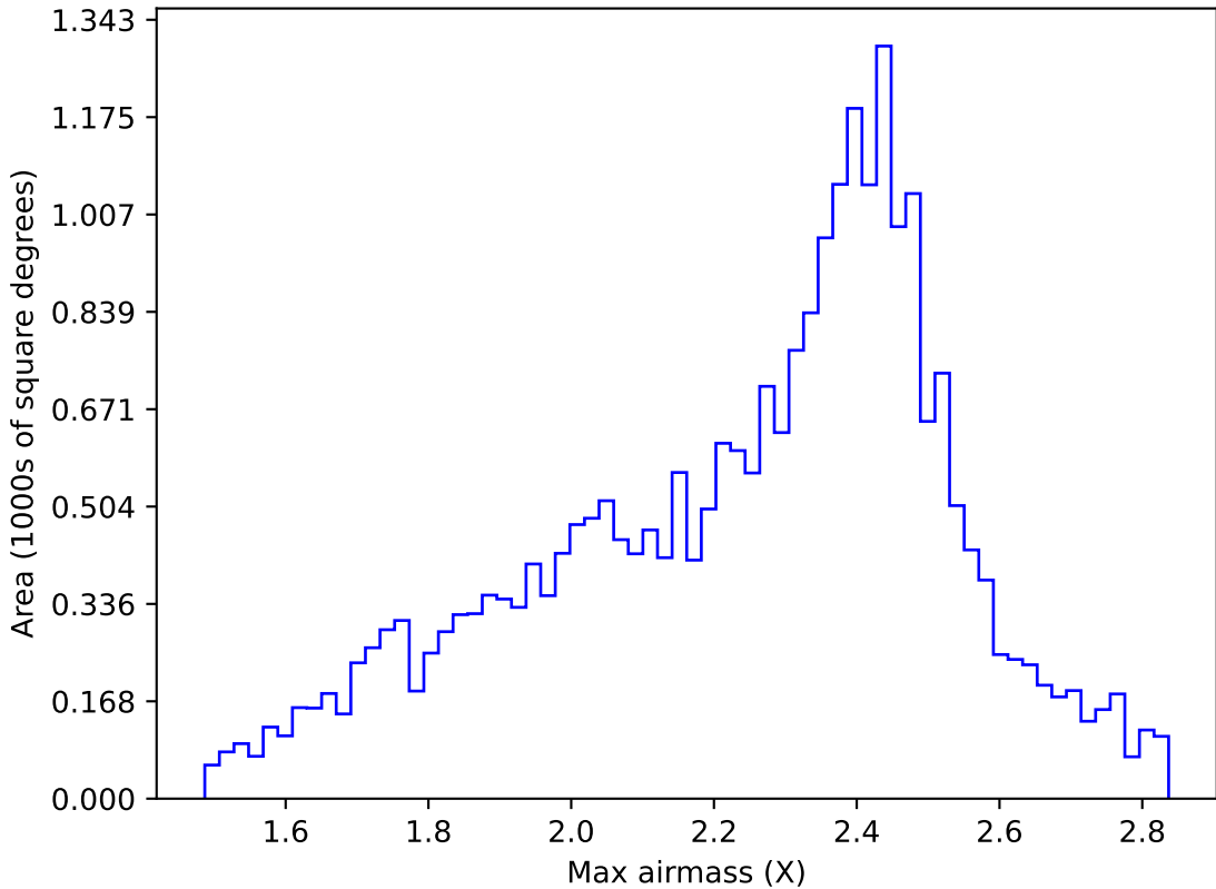
ddf_loaded_half_fl15_v3.4_10yrs All sky r band: Max airmass
