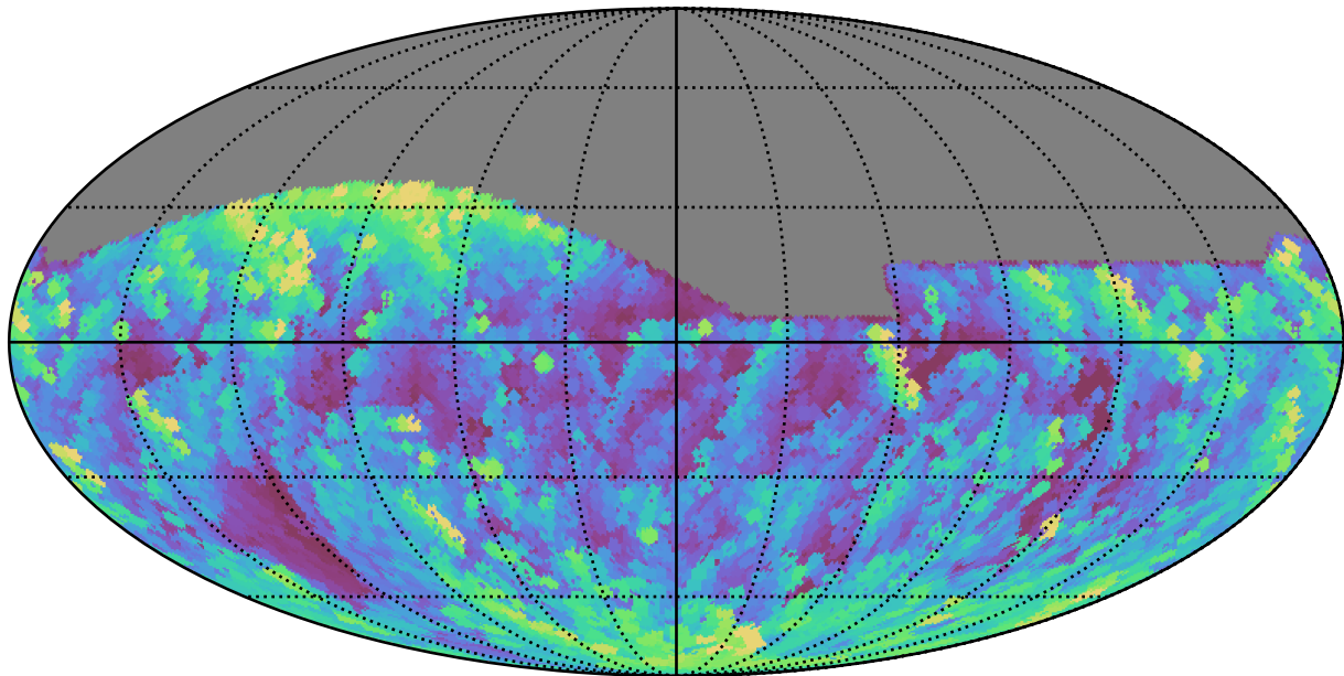
ddf_loaded_half_fl15_v3.4_10yrs All sky g band: Max airmass
