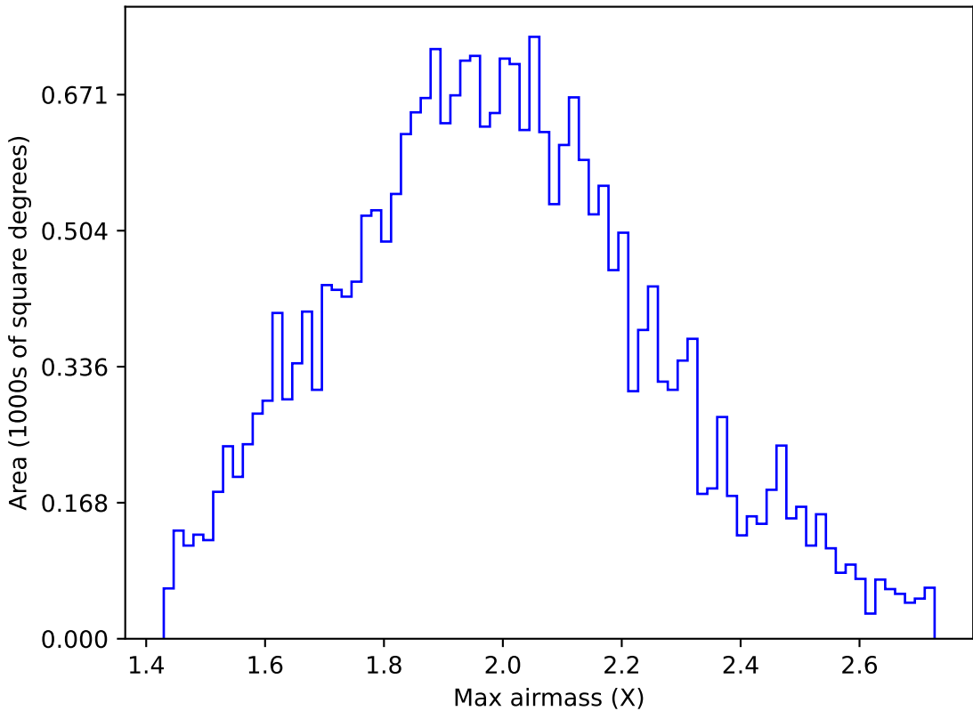
ddf_loaded_half_fl15_v3.4_10yrs All sky g band: Max airmass
