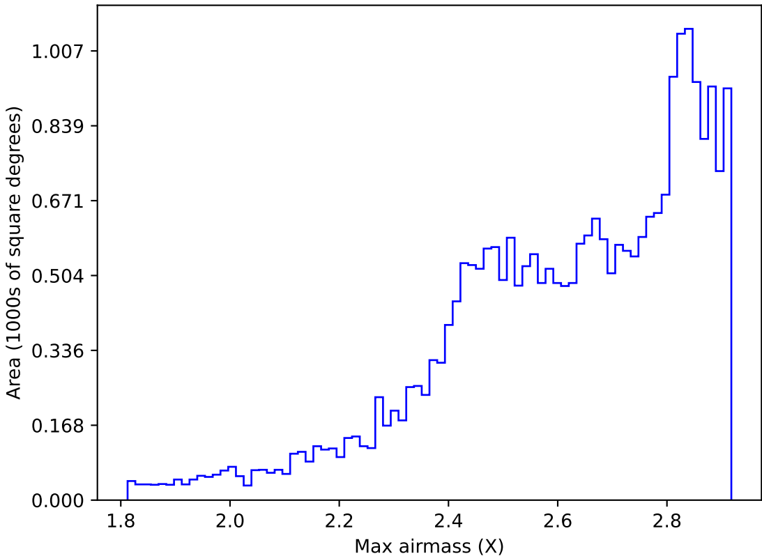
ddf_loaded_half_fl15_v3.4_10yrs All sky all bands: Max airmass
