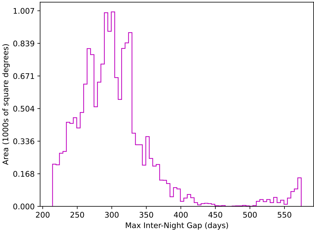
ddf_loaded_half_fl15_v3.4_10yrs WFD z band: Max Inter-Night Gap
