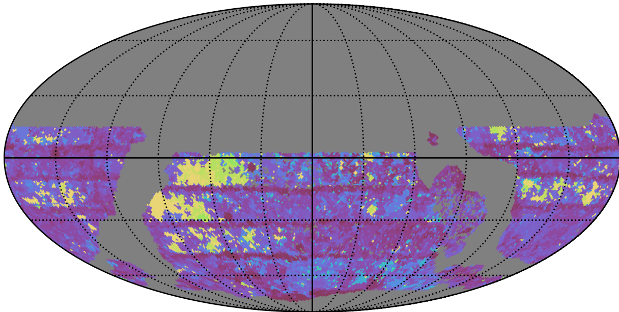
ddf_loaded_half_fl15_v3.4_10yrs WFD y band: Max Inter-Night Gap
