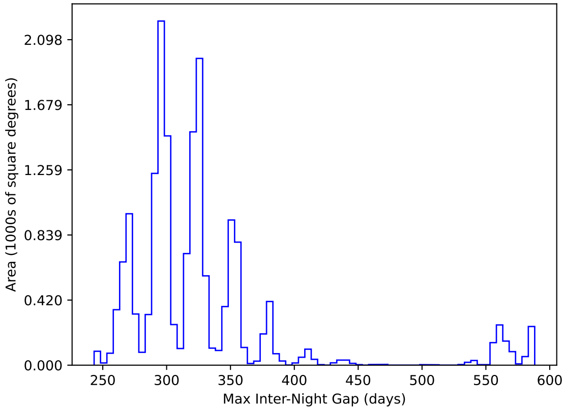
ddf_loaded_half_fl15_v3.4_10yrs WFD y band: Max Inter-Night Gap
