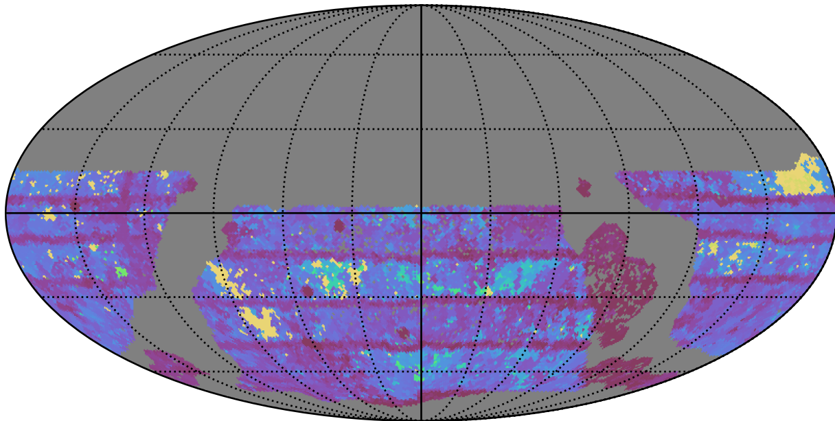
ddf_loaded_half_fl15_v3.4_10yrs WFD r band: Max Inter-Night Gap
