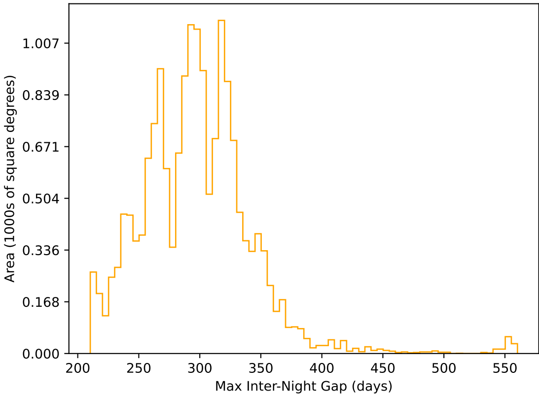
ddf_loaded_half_fl15_v3.4_10yrs WFD r band: Max Inter-Night Gap
