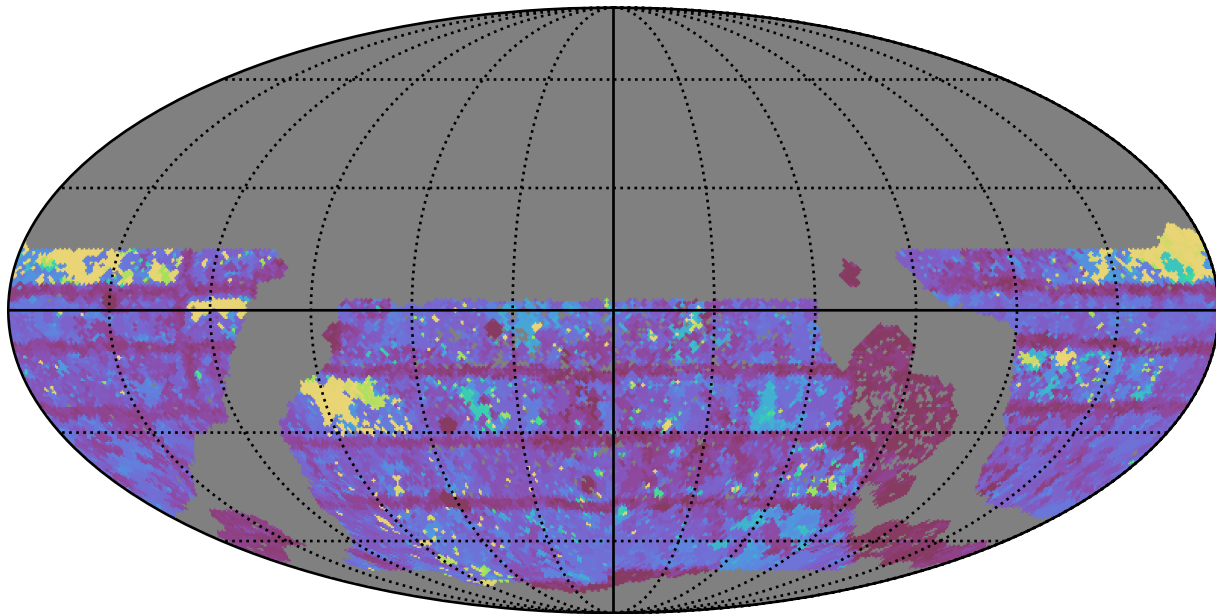
ddf_loaded_half_fl15_v3.4_10yrs WFD i band: Max Inter-Night Gap
