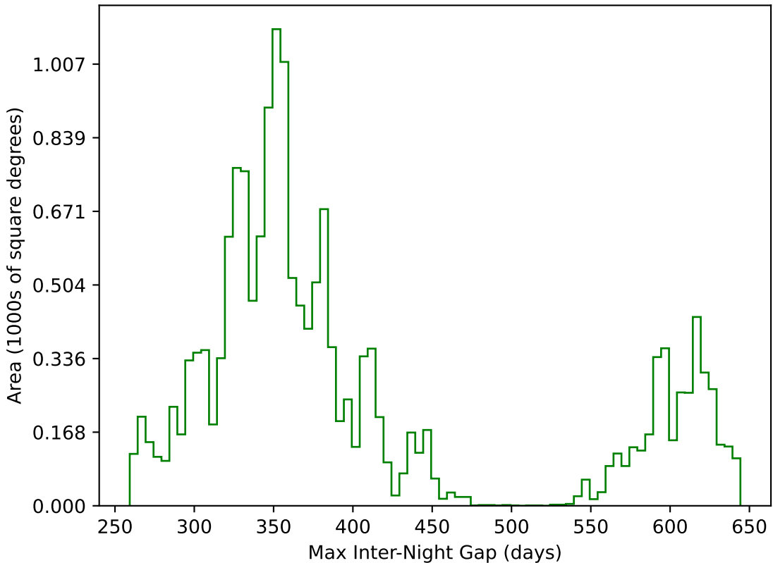
ddf_loaded_half_fl15_v3.4_10yrs WFD g band: Max Inter-Night Gap
