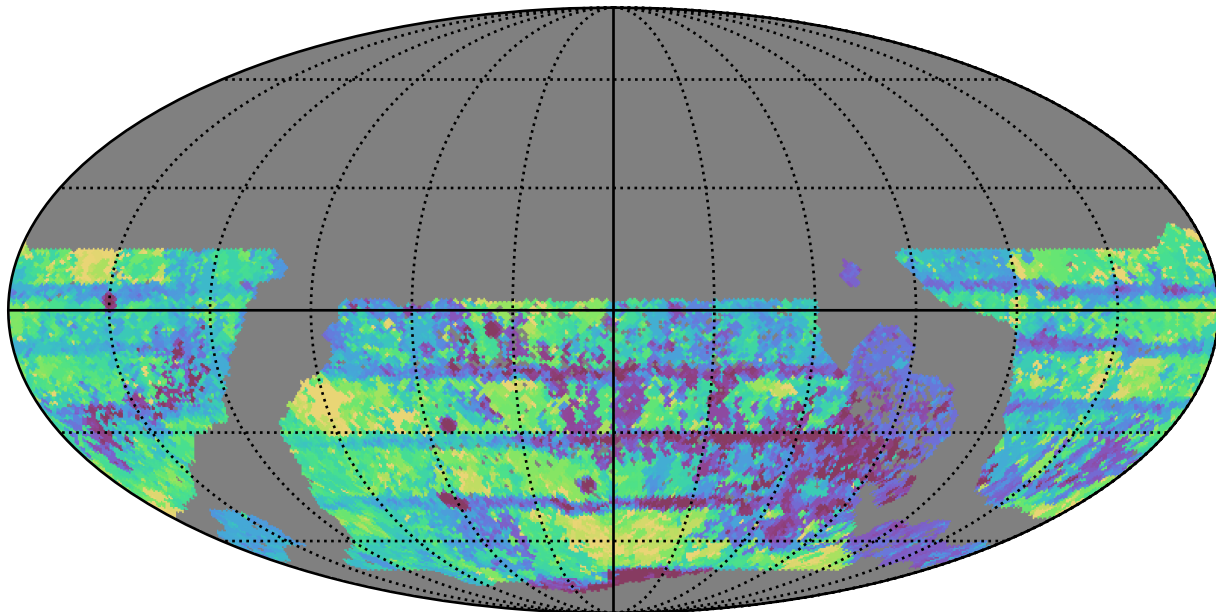
ddf_loaded_half_fl15_v3.4_10yrs WFD all bands: Max Inter-Night Gap
