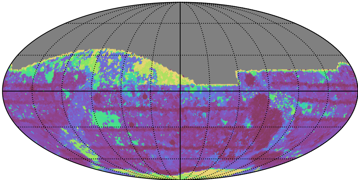
ddf_loaded_half_fl15_v3.4_10yrs All sky z band: Max Inter-Night Gap
