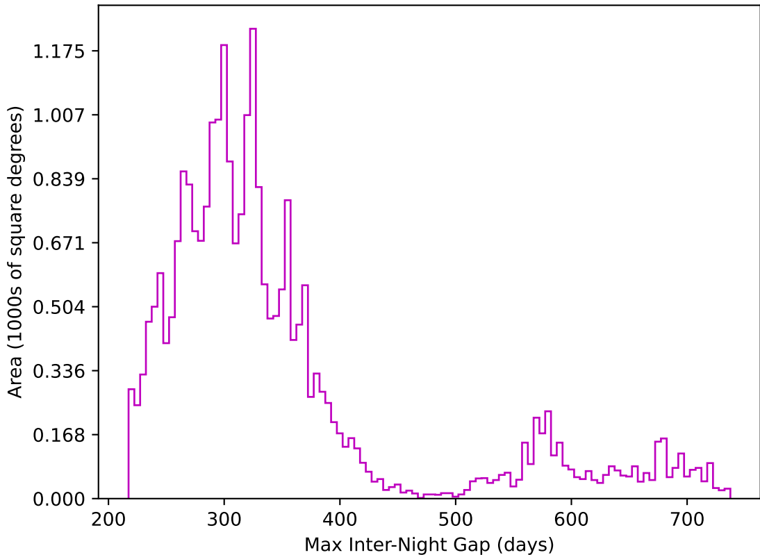
ddf_loaded_half_fl15_v3.4_10yrs All sky z band: Max Inter-Night Gap
