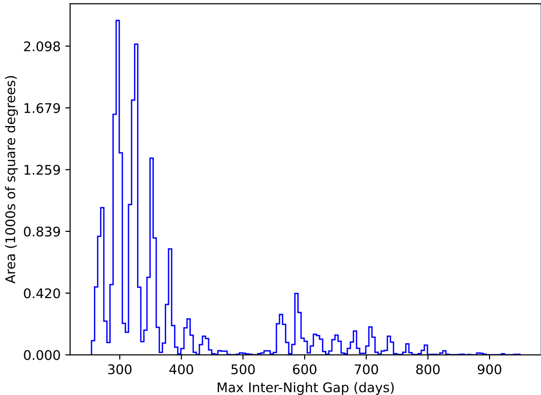
ddf_loaded_half_fl15_v3.4_10yrs All sky y band: Max Inter-Night Gap
