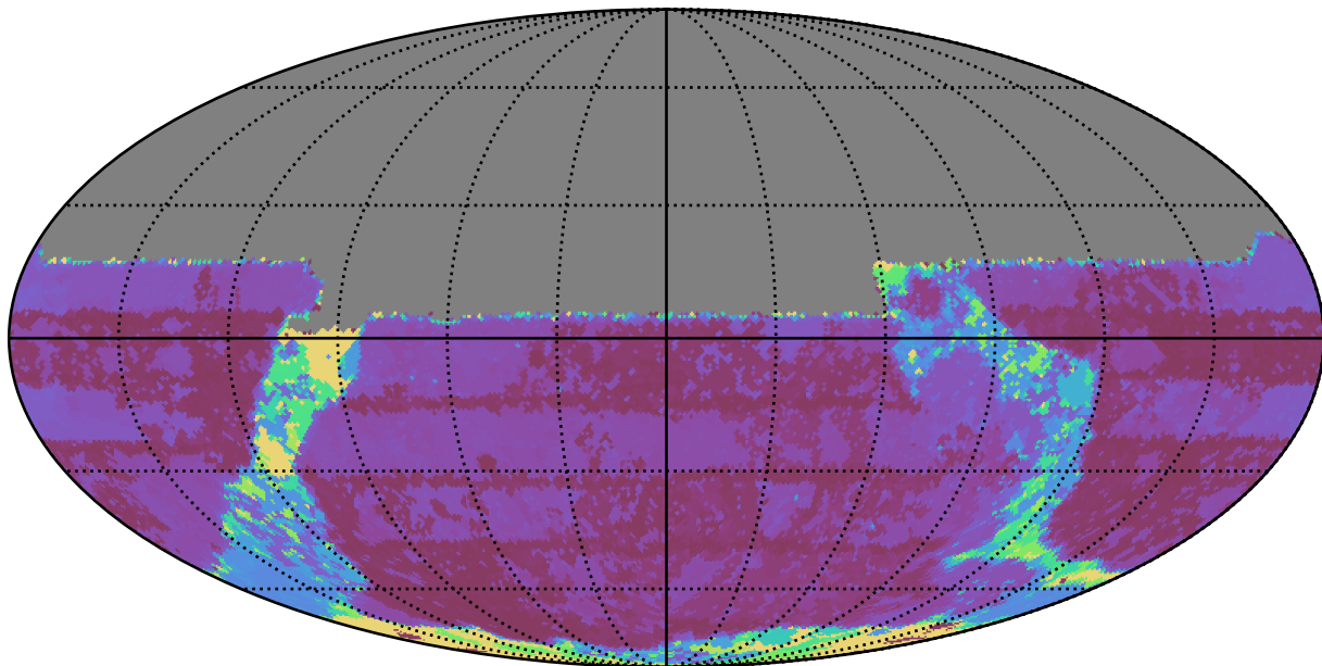
ddf_loaded_half_fl15_v3.4_10yrs All sky u band: Max Inter-Night Gap
