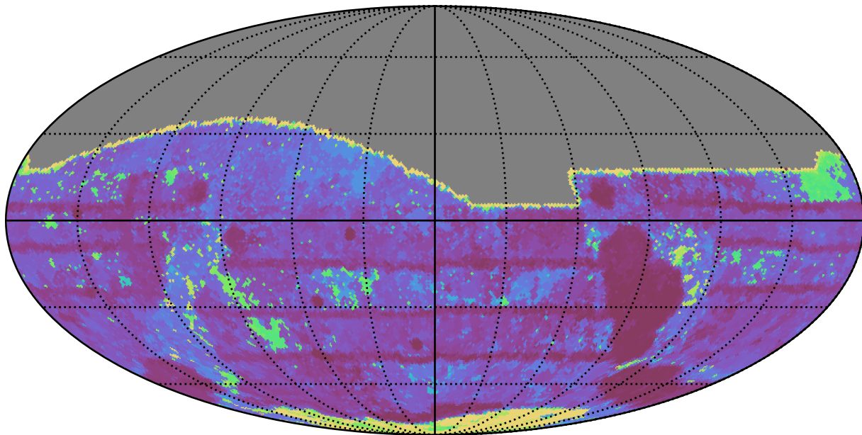
ddf_loaded_half_fl15_v3.4_10yrs All sky r band: Max Inter-Night Gap
