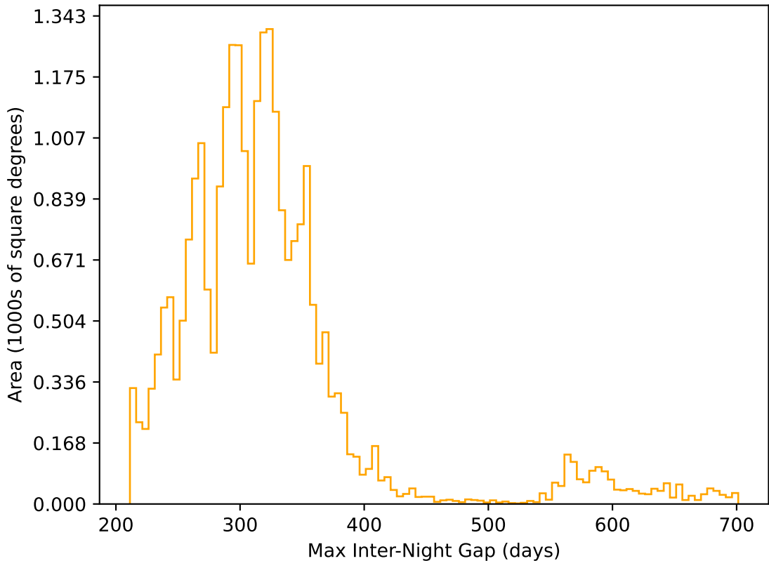
ddf_loaded_half_fl15_v3.4_10yrs All sky r band: Max Inter-Night Gap
