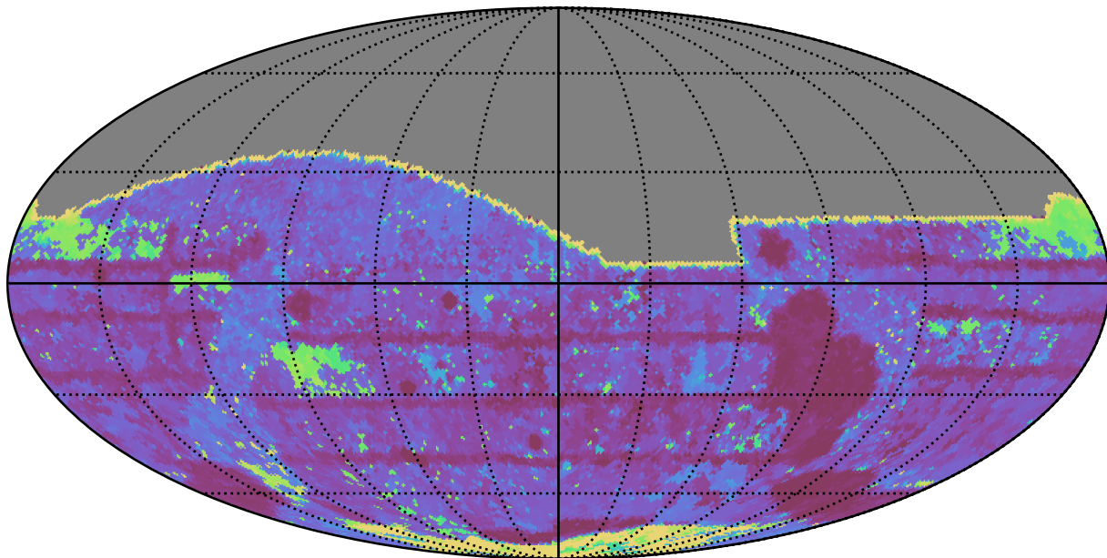
ddf_loaded_half_fl15_v3.4_10yrs All sky i band: Max Inter-Night Gap
